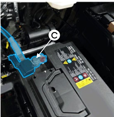
C. Disconnect the 12V auxiliary battery negative(-) terminal.
